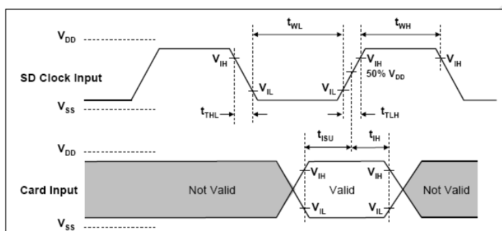
Card Input Timing (High Speed Card)
